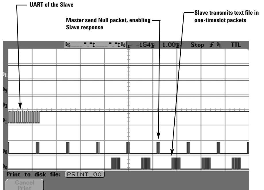
Figure 7: File transmission from the Slave
