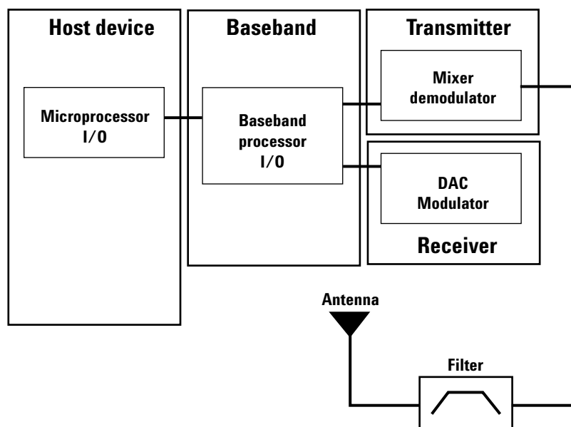
Figure 1: Bluetooth device functional blocks
