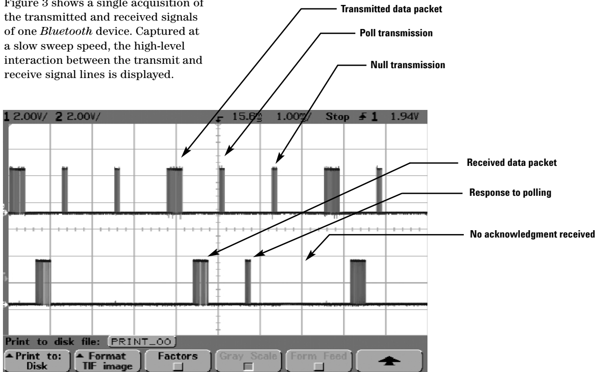
Figure 3: Transmit and receive high-level view
