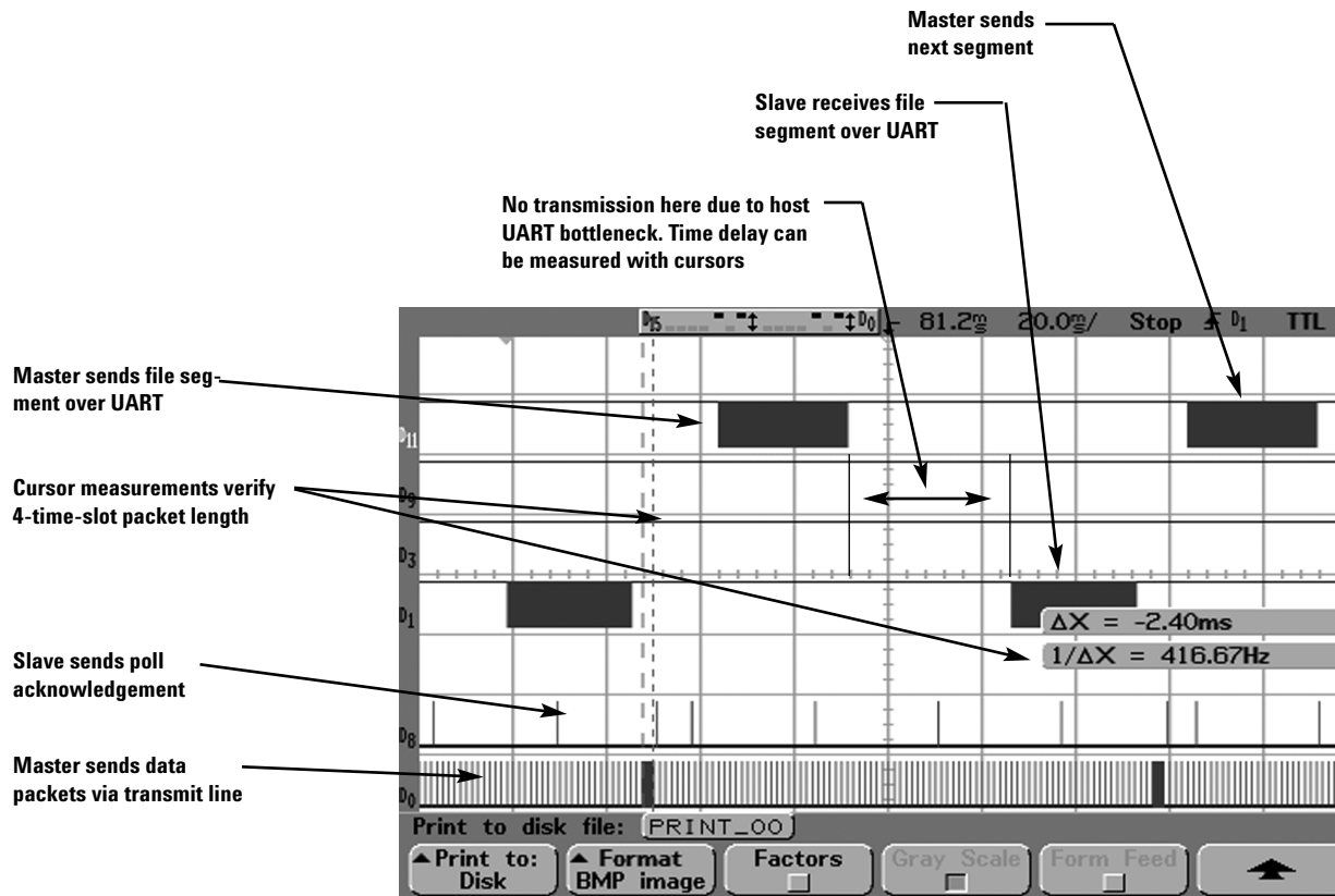
Figure 6: Master transfers file over UART
