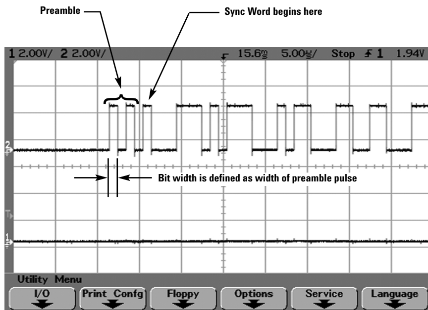
Figure 4: Transmitted data packet zoomed view
