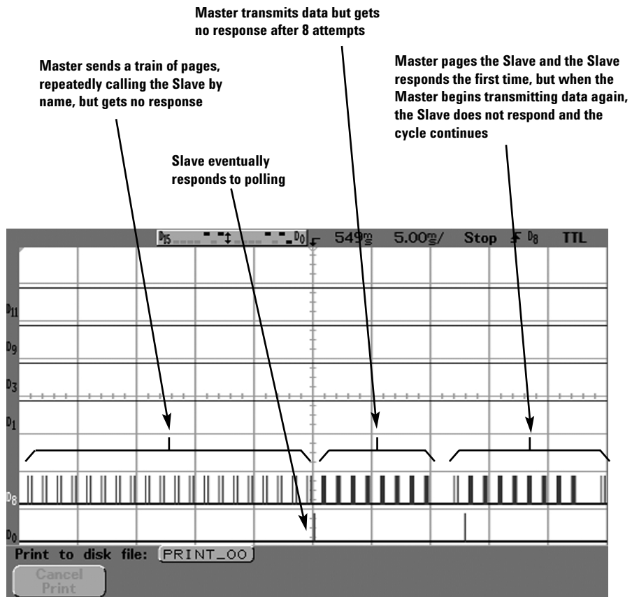
Figure 8: Software logic error occurs
