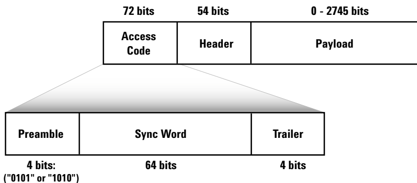
Figure 5: Bluetooth packet structure specification
